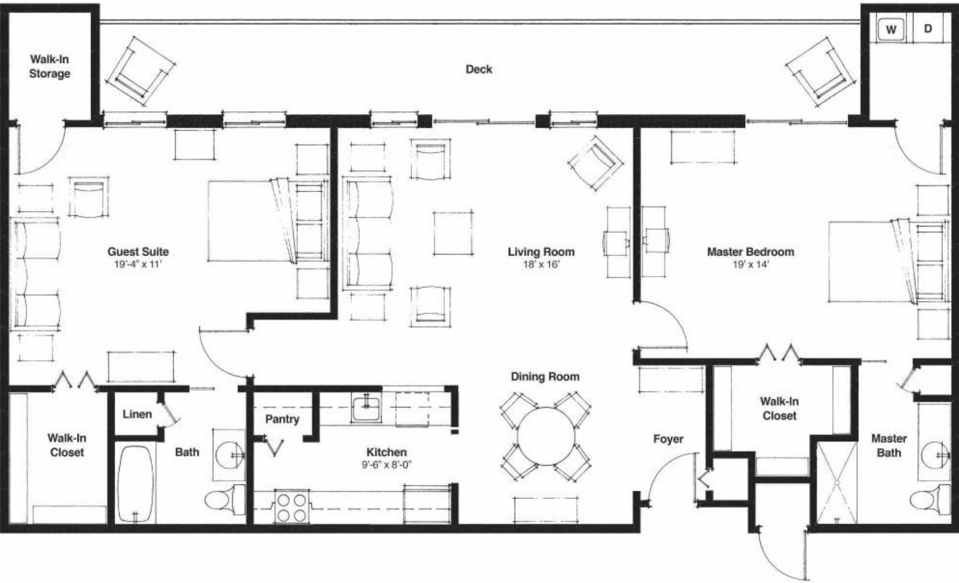
Erskine E • Two Bedroom / Two Bath 1453 sq ft
